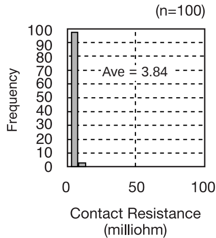
N.O. contact - Distribution of contact resistance
